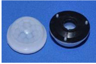
Model: 023115 Size: \varnothing 26*17.3 Focal: 11.5mm Angle: 120 ° Distance: 10m
