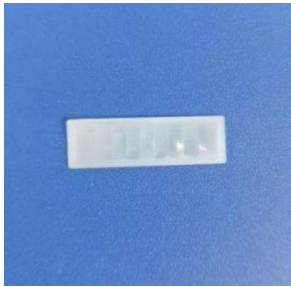
Model: SB-3611 Size: 35.3 *10.7 Focal: 7mm Angle: 120 ° Distance: 6m
