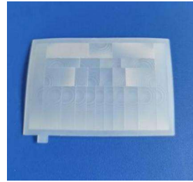
Model: 86000 Size: 41.7*60 Focal: 30mm Angle: 90 ° Distance: 15m
