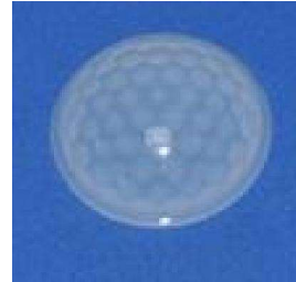
Model: 8605-2B Size: \varnothing 35.7* 11.5 Focal: 15mm Angle: 360 ° Distance: \varphi 10m
