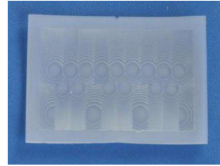
Model: 7704-3 Size: 56.7 *35.7 Focal: 23mm Angle: 110 ° Distance: 12m
