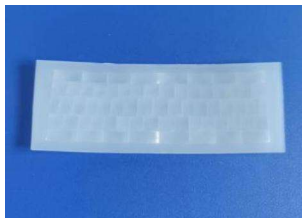
Model: 8501-5 Size: 76*36.2 Focal: 20mm Angle: 120 ° Distance: 10m
