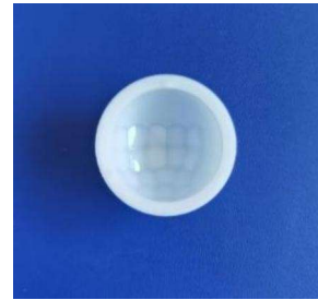
Model: YY-023115-15 Size: \varnothing 26 Focal: 11.5mm Angle: 120^\circ Distance: r/R 10m
