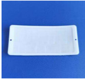
Model: WL-NK-04 Size: 54*25 Focal: 12mm Angle: 120 ° Distance: 8m
