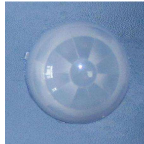
Model: PN-08-4G Size: 15.21* 14.95*5.48 Focal: 4mm Angle: 90 ° Distance: 3m
