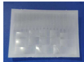
Model: YY-DWA-V2 Size: 42.6 *61 Focal: 30.5mm Angle: 101 ° Distance: 9m
