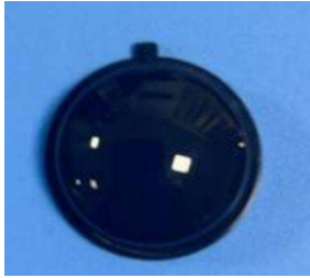
Model: 13120F-4 Size: \Phi 14.2 Focal: 6mm Angle: 120 ° Distance: 6m
