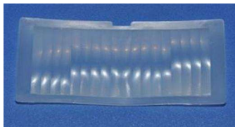
Model: 7707-1A Size: 91.3 *39.5 Focal: 25mm Angle: 180 ° Distance: 16m
