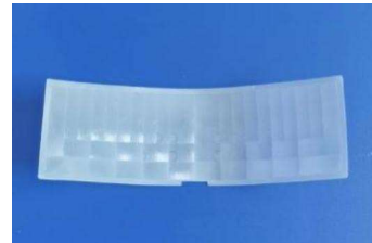
Model: AF-2430 Size: 116.5*38 Focal: 30mm Angle: 180 ° Distance: 20m Double PIR
