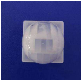
Model: YY-1003-45 Size: 24 \times 24 Focal: 12mm Angle: 120^\circ Distance: 10m
