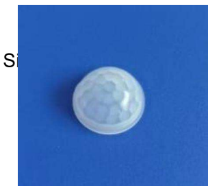
Model: YY-1608 Size: Ø17.5 Focal: 7mm Angle: 120 ° Distance: 6m
