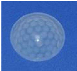
Model: 8603-4A Size: \varnothing 35.6*11 Focal: 17.5mm Angle: 360 ° Distance: Dia. 12m
