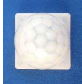
Model: 024120 (without leg) Size: 23.5*23.5*17.2 Focal: 12mm Angle: 120 ° Distance: 12m
