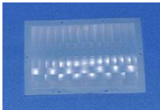
Model: 614230 Size: 60.7 *42.4 Focal: 30.5mm Angle: 90 ° Distance: 12m
